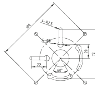
Mounting dimensions in mm
